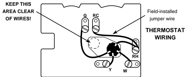
Figure 6. Cool only, 3-wire, single transformer systems
