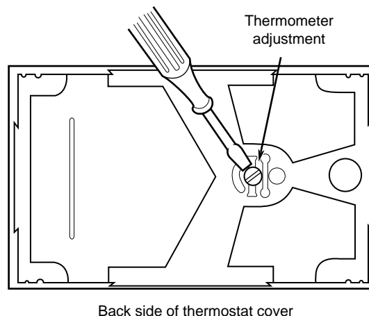
Figure 13. Calibrating Thermostat Thermometer
