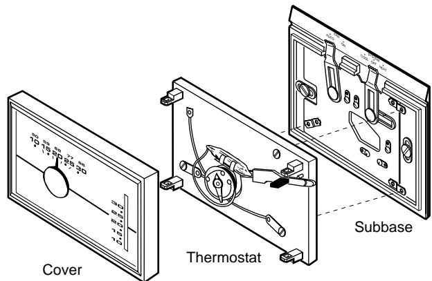
Figure 9. Attach Thermostat to Subbase
