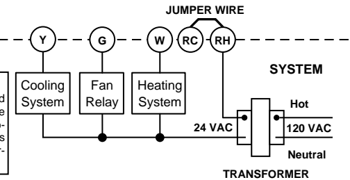
Figure 7. Heat/cool, 4-wire, single transformer systems
