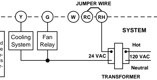
Figure 6. Cool only, 3-wire, single transformer systems
