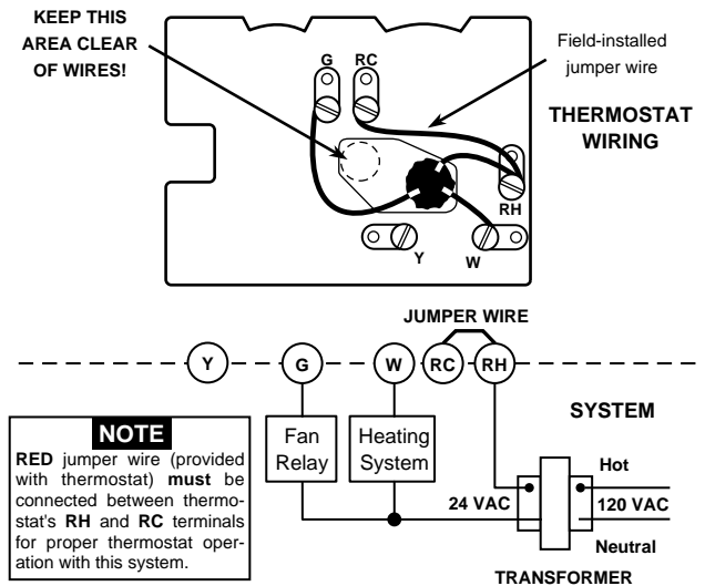
Figure 5. Heat-only, 3-wire, single transformer systems
