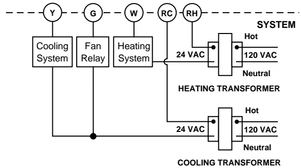
Figure 8. Heat/cool, 5-wire, two-transformer systems
